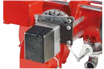
Example of servomotor and air damper of GAS 3 P/M
